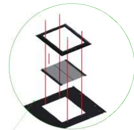
Brush Cable Entry
