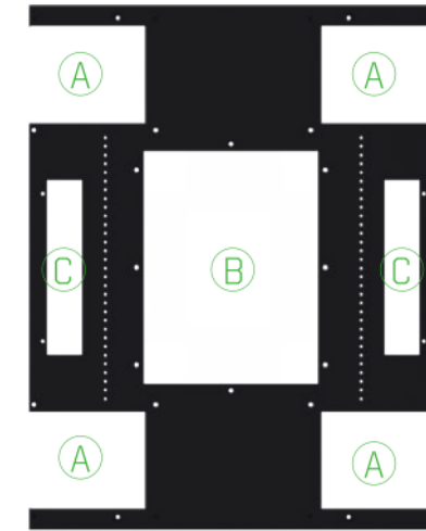
Standard Plain Roof Plus
